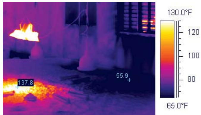
Figure 2. Draft from loose fan shutter
