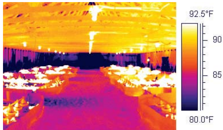
Figure 5. Draft moving towards the center of the barn from between brooder rings
