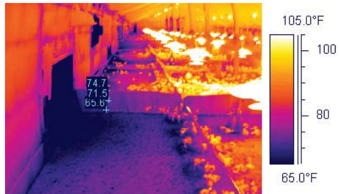
Figure 1. Draft from loose-fitting door
