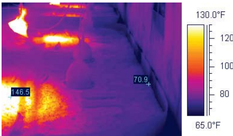
Figure 6. Brooder ring up against sidewall
